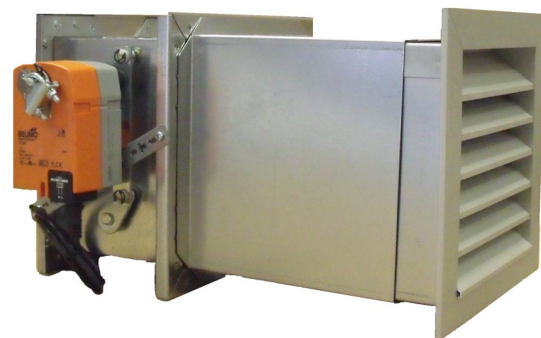
Air Make up Damper with Telescopic Duct and Weather Louvre
